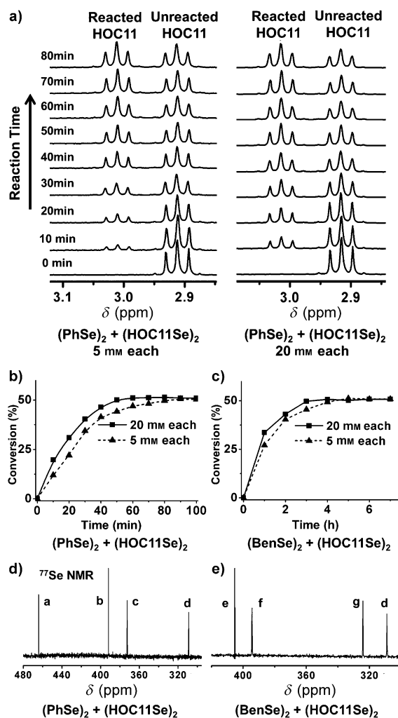
Figure 1. ^1\text{H} NMR and ^{77}\text{Se} NMR data obtained during diselenide exchange. The conversion of the reaction was determined in terms of the amount of reacted (\text{HOC11Se})_2 . a) After exchange with (\text{PhSe})_2 , the peak corresponding to the \text{CH}_2\text{Se} protons in (\text{HOC11Se})_2 shifted from 2.91 ppm to 3.01 ppm. b) Dependence of the conversion of the exchange reaction between (\text{PhSe})_2 and (\text{HOC11Se})_2 on the concentration. c) Dependence of the conversion of the exchange reaction between (\text{BenSe})_2 and (\text{HOC11Se})_2 on the concentration. The reaction proceeds faster at a higher concentration. d, e) The ^{77}\text{Se} NMR spectra after the reaction. Peaks a (464.1 ppm) and d (309.0 ppm) belong to (\text{PhSe})_2 and (\text{HOC11Se})_2 ; peak e (405.3 ppm) belongs to (\text{BenSe})_2 ; peaks b (391.9 ppm) and c (372.6 ppm) belong to the exchange product (\text{HOC11Se})(\text{SePh}) ; peaks f (394.4 ppm) and g (324.2 ppm) belong to the exchange product (\text{HOC11Se})(\text{SeBen}) . See the Supporting Information for full ^1\text{H} NMR spectra.
